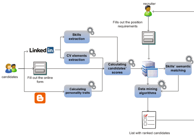
Fig. 1. System’s Architecture
